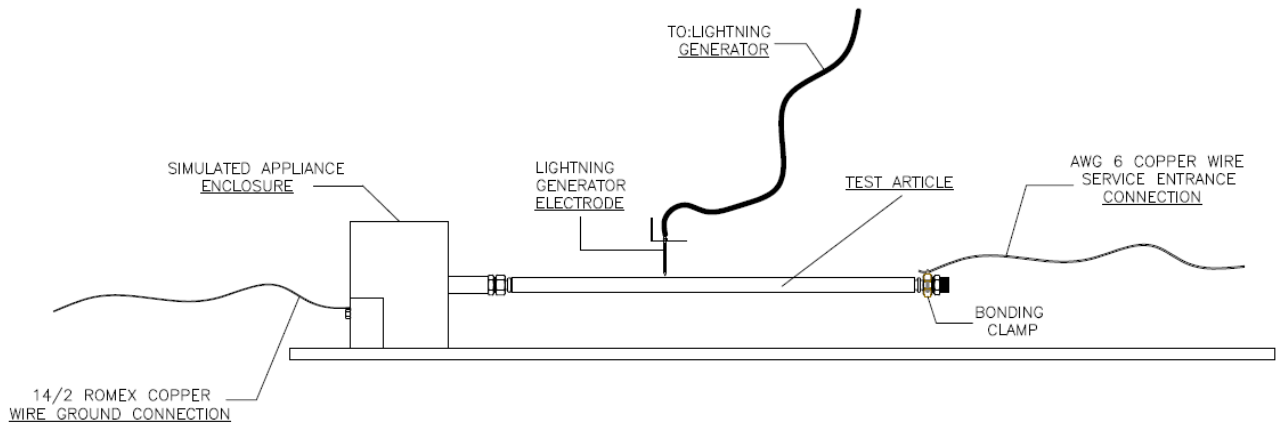
FIGURE 3—TEST SCHEMATIC
