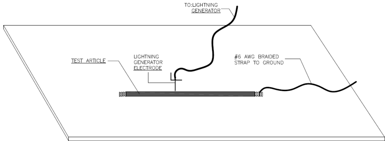
FIGURE 2—TEST SCHEMATIC
